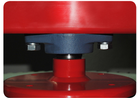
SKFY-bearing units with oval flanged housing mounted in fruit tree cutting bar machine
